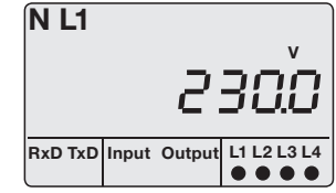
Fig. Display example for "Display mode", measured value displayed: U_{L1-N} = 230.0V .
