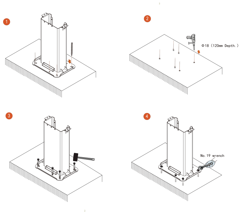
figure 2-21 Pole installation
