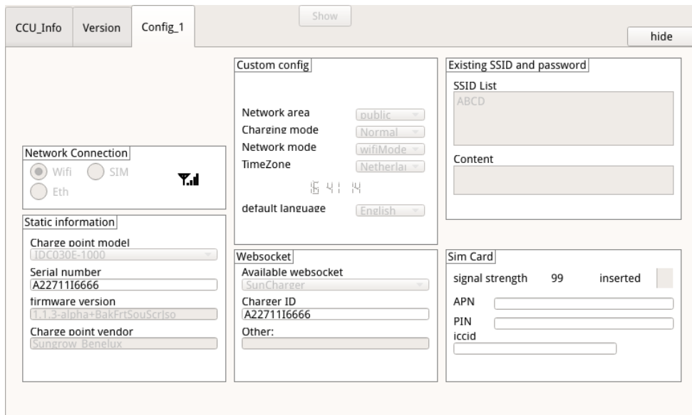
figure 4-12 Administrator page
