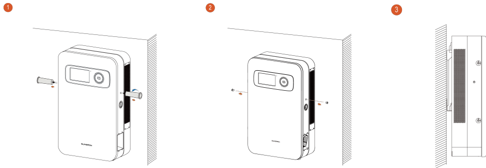
figure 2-11 Installation of the keyhole plug
