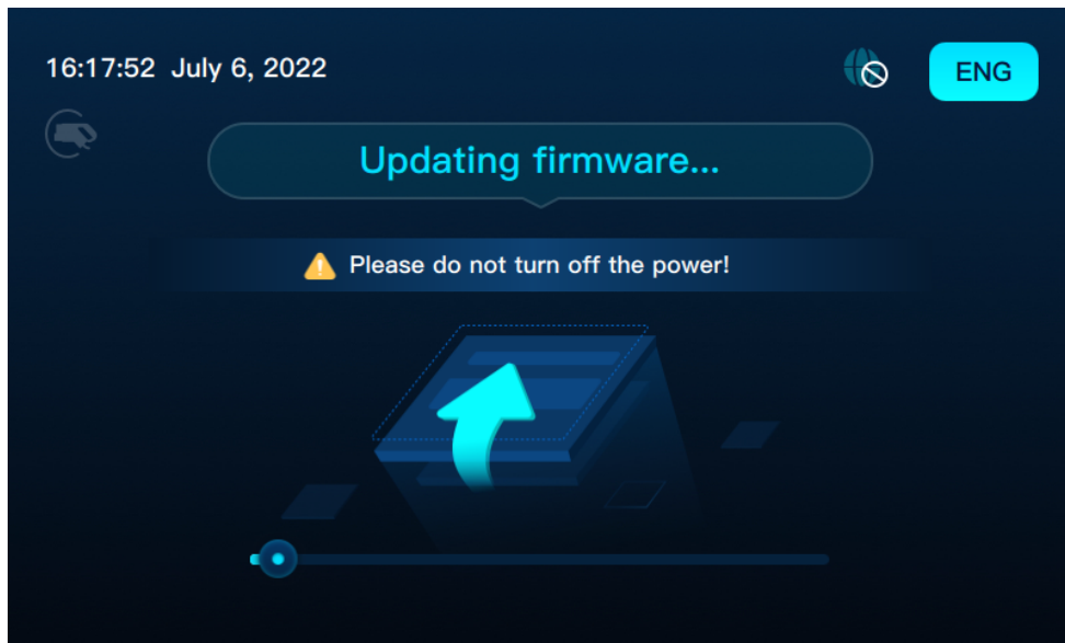
figure 3-10 Firmware Update
